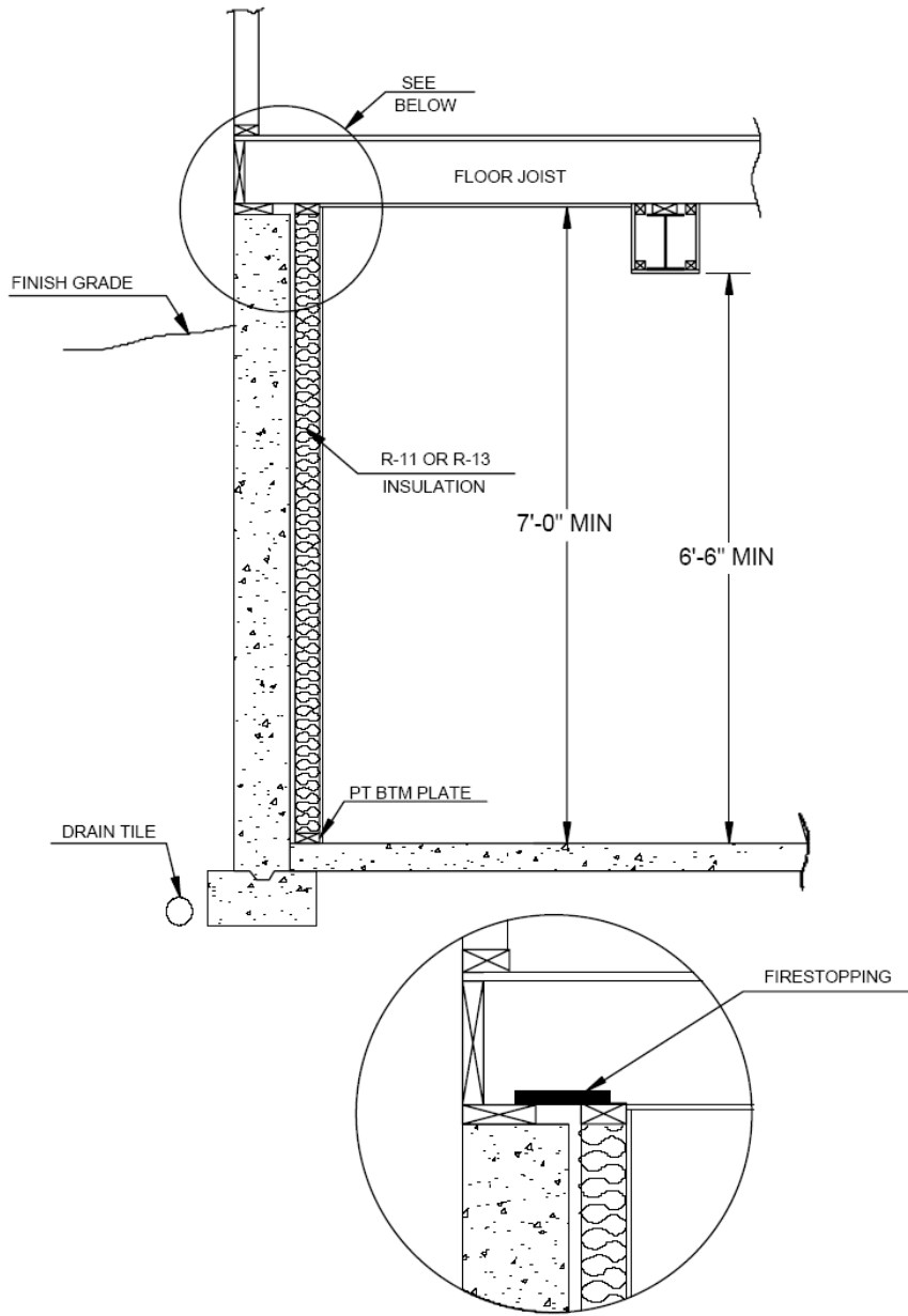
TYPICAL ELEVATION
